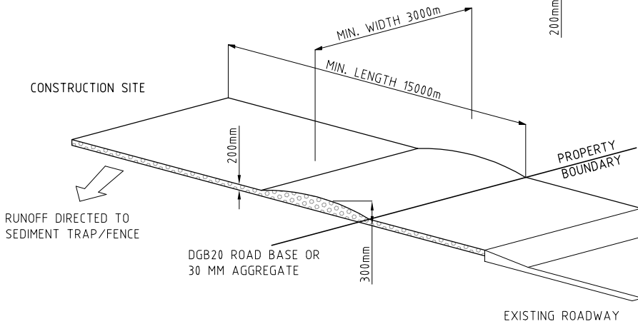
SITE ACCESS DETAIL NTS
